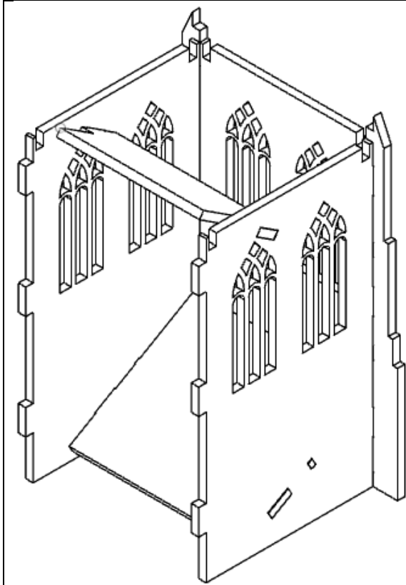
5 Glue on the rear face
