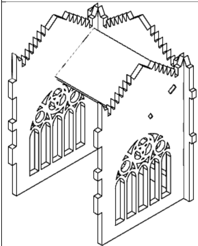
11 Glue on the rear face, keeping the textured side facing outward
