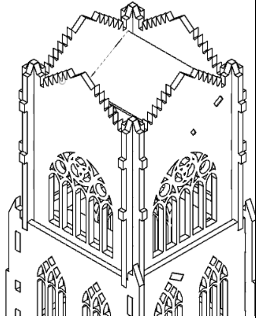
14 Glue on the top section to the bottom half. The buttresses should slot into the channels on the top of the lower section.
