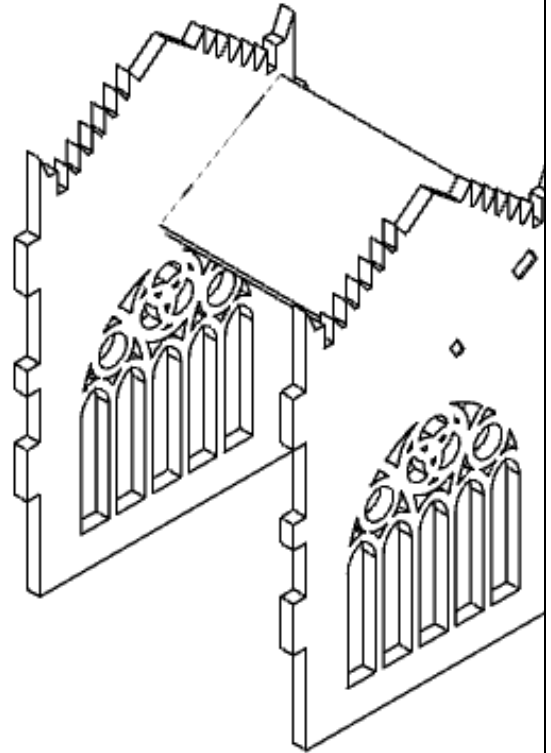
10 Glue on the opposite side, keeping the textured side facing outward
